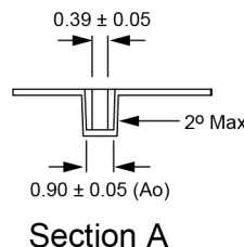
Figure 5A. SC-79 (SMS7621-079LF) Tape and Reel Dimensions
