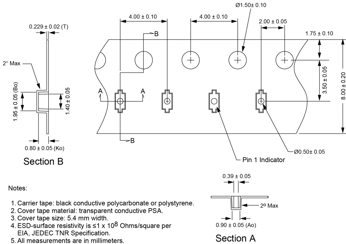
Figure 5B. SC-79 (SMS7630-079LF) Tape and Reel Dimensions
