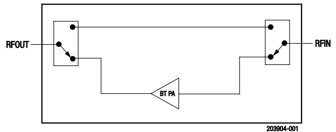
Figure 1. SKY85018-11 Block Diagram
