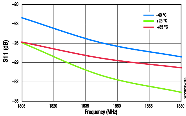
Figure 15. Input Return Loss vs Frequency Across Temperature (Small Signal, P_{IN} = -20 dBm)
