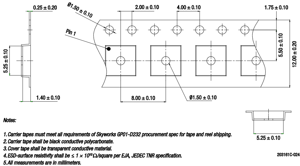
Figure 24. SKY66291-11 Tape and Reel Dimensions
