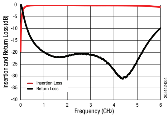
Figure 4. Small Signal Performance
