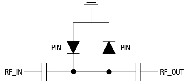
Figure 1. SKY16603-632LF Block Diagram
