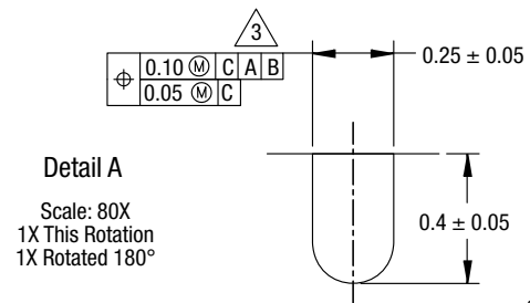
Figure 11. SKY16603-632LF Package Dimensions
