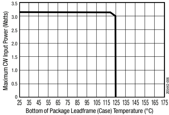
Figure 6. Power Derating Curve ( P_d = 0.4\text{ W @ }120^{\circ}\text{C} ) v Package Leadframe (Case) Temperature
