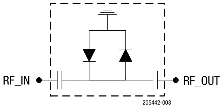
Figure 3. SKY16603-632LF Schematic
