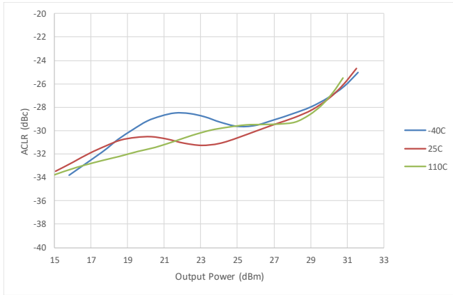
Figure 3. ACLR vs. Output Power Over Temperature (PAR = 8.5 dB, 100 MHz Signal)
