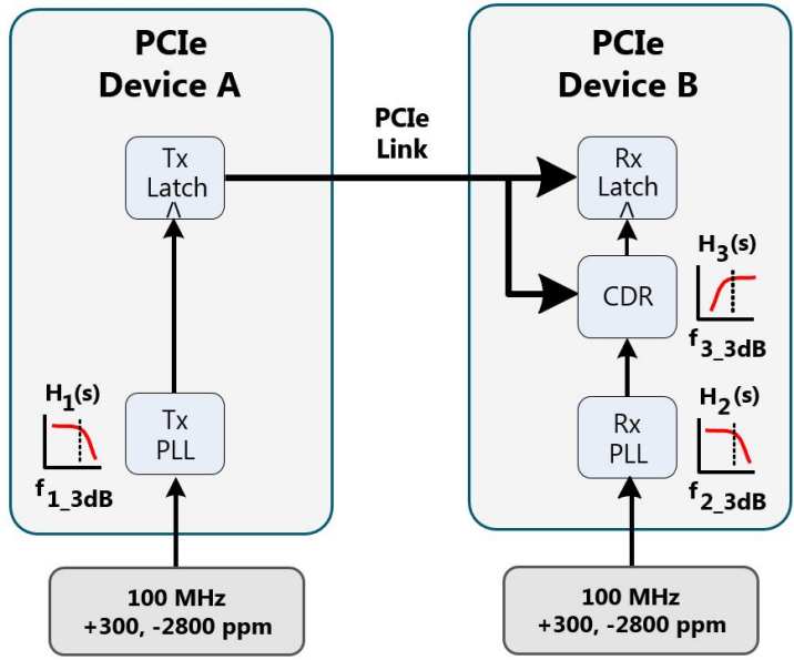
Figure 2.2. SRNS/SRIS Clock Architecture
