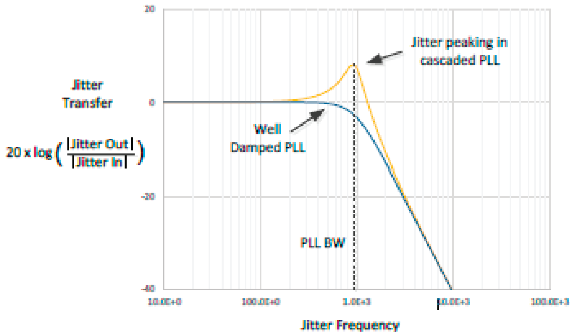
Figure 2. PLL Based Jitter Tracking and Filtering
