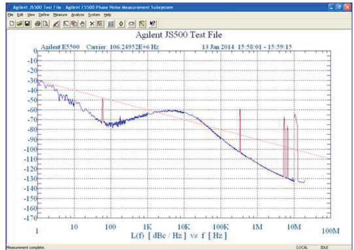
Figure 1. Example Sub-optimal PLL-based XO Phase Noise and Period Jitter
