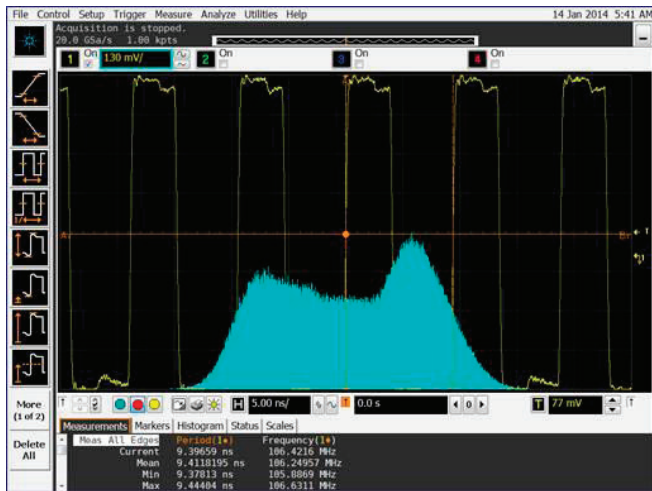
Figure 1. Example Sub-optimal PLL-based XO Phase Noise and Period Jitter
